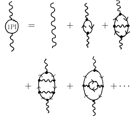
Fig. 41.2 Some contributions to the Green’s function i\tilde{\Pi}^{\mu\nu}(q) .
