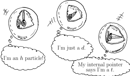
Fig. 13.1 In our toy model, particles can be imagined as having an internal dial. Whether the dial points along (1, 0, 0) , (0, 1, 0) or (0, 0, 1) determines which kind of particle it is. The position of the dial is not related to the directions in spacetime through which particles move, but expresses a direction in abstract space describing the internal symmetry.
