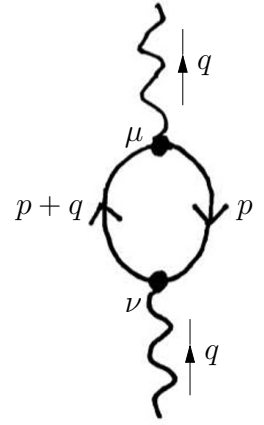
Fig. 41.5 The photon propagator with a single electron-hole loop insertion.
