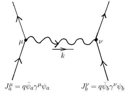
Fig. 39.1 The exchange of a virtual photon.
