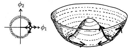
Fig. 26.7 Breaking symmetry at the position (\phi_1, \phi_2) = \left(+\sqrt{\frac{6\mu^2}{\lambda}}, 0\right) . There are two possible excitations: the particle can oscillate up and down in the \phi_1 direction (a massive excitation) or trundle round in the gutter (a massless excitation).
