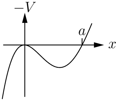
Fig. 50.9 The barrier potential turned upside-down.
