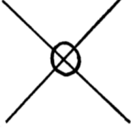
Fig. 32.2 The C -counterterm.
