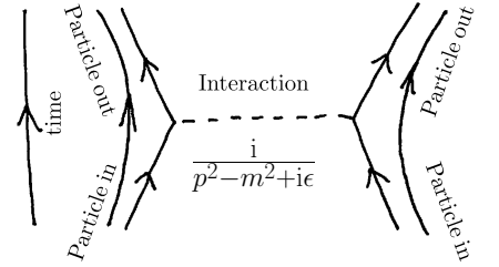
Fig. 17.5 A Feynman diagram for two particles scattering. The amplitude for the process includes a factor i/(p^2 - m^2 + i\epsilon) , which describes the propagation of a virtual, force-carrying particle which can be thought of as mediating a Yukawa force.
