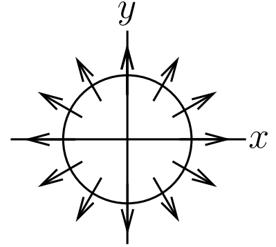
Fig. 29.11 Fields at large distances for an n = 1 vortex.
