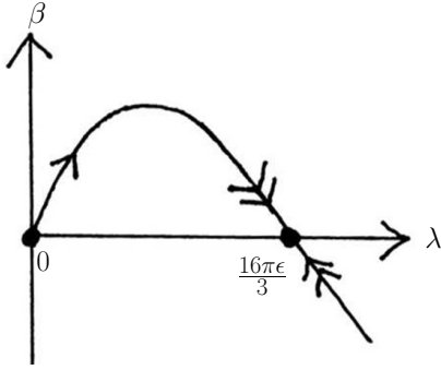
Fig. 35.3 The \beta function for the behaviour of the coupling constant \lambda .
