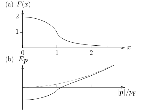
Fig. 43.4 (a) The function F(x) . (b) The energy of an electron in the Hartree–Fock approximation E_{\mathbf{p}} = \frac{p^2}{2m} + \Sigma_{\mathbf{p}}^{(F)} .
