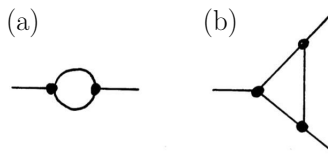
Fig. 32.5 Two divergent diagrams occurring in \phi^3 theory.
