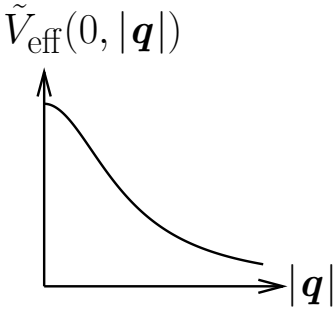
Fig. 43.15 The static effective potential \lim_{|\mathbf{q}| \rightarrow 0} \tilde{V}_{\text{eff}}(0, \mathbf{q}) .
