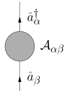
Fig. 4.1 A process represented by the operator in eqn 4.18.
