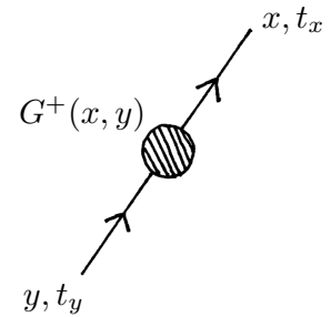
Fig. 16.1 A cartoon representation of the propagator. It will turn out to be the basic unit of the Feynman diagram.
