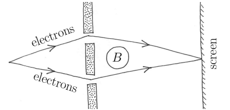
Fig. 29.4 The Aharonov–Bohm effect. Electrons diffract through two slits but their paths enclose a solenoid. The field inside the solenoid is B , but the electrons only pass through regions in which there is no magnetic field.
