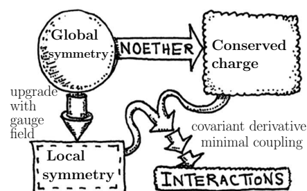
Fig. 38.4 The minimal coupling prescription in QED.
