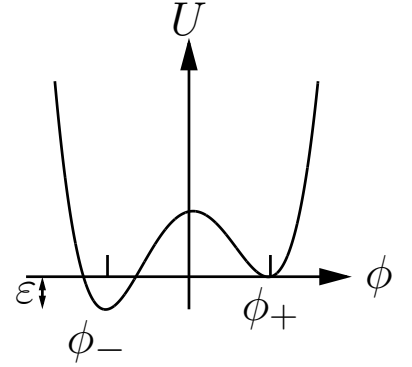
Fig. 50.12 False vacuum potential.
