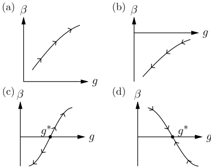
Fig. 34.2 Four examples of flows in a configuration space defined by a single coupling constant g , visualized by plotting \beta(g) = \frac{dg}{db} . Arrows show the direction that the length scale \ell \rightarrow \infty .
