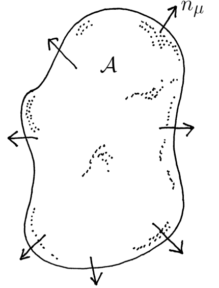
Fig. 10.1 A region of spacetime with surface \mathcal{A} . The outward normal is n_\mu .
