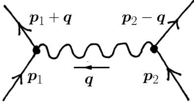
Fig. 4.8 A Feynman diagram for the process described in the text. Interpreting this diagram, one can think of time increasing in the vertical direction.
