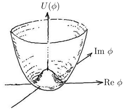
Fig. 47.1 The potential of the Higgs field.
