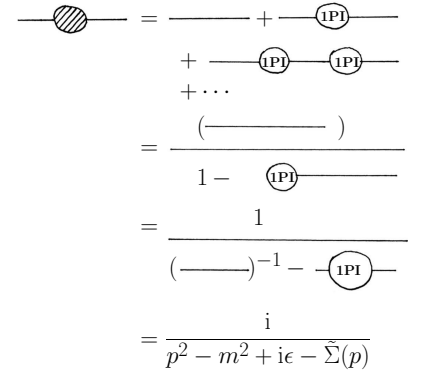
Fig. 33.4 Diagrammatic version of eqn 33.6
